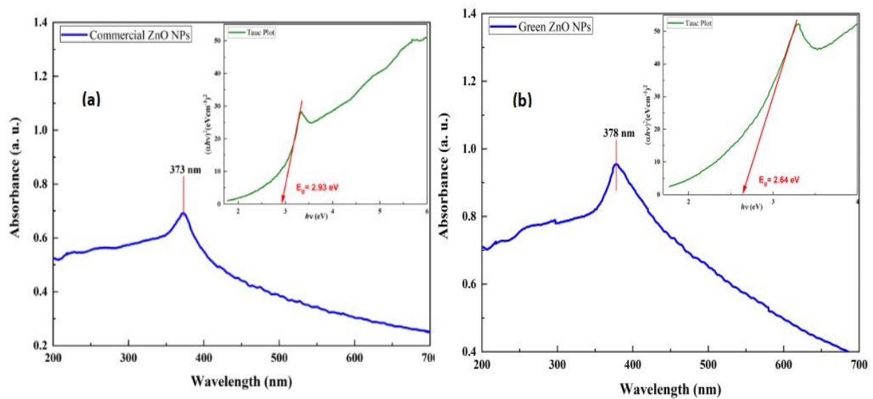
Fig.8. UV-Vis absorption spectra and corresponding Tauc plots of (a) commercial ZnO nanoparticles and (b) green-synthesized ZnO nanoparticles.
