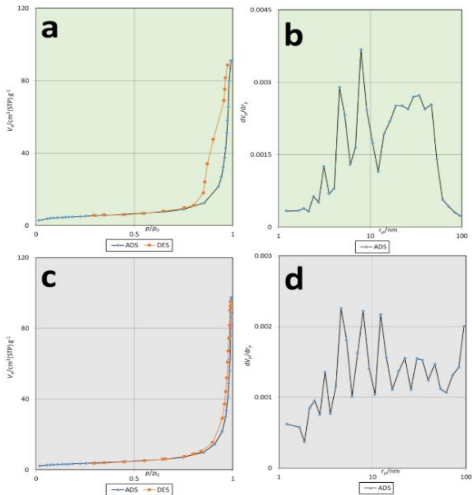
Fig.5. Nitrogen adsorption–desorption and BJH pore-size distribution of ZnO samples: (a, b) commercial ZnO nanoparticles and (c, d) green-synthesized ZnO nanoparticles.
