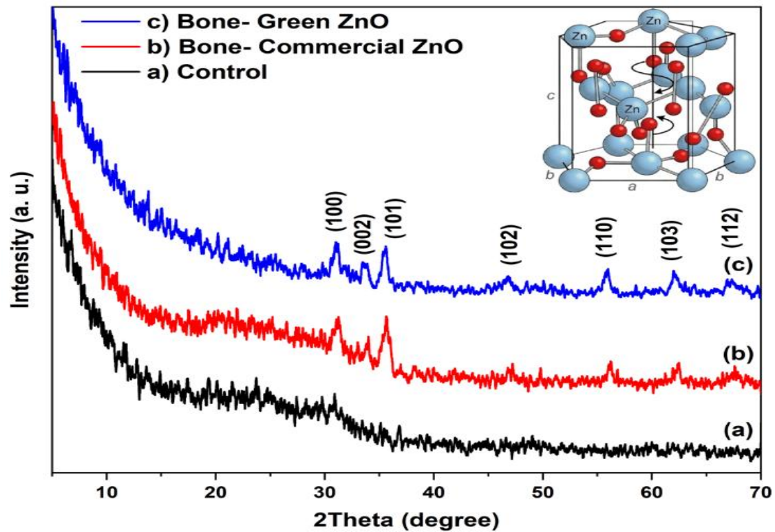
Fig.7. X-ray diffraction (XRD) patterns of (a) uncoated cortical bone plate (control), (b) bone plate coated with commercial ZnO nanoparticles, and (c) bone plate coated with green-synthesized ZnO nanoparticles.
