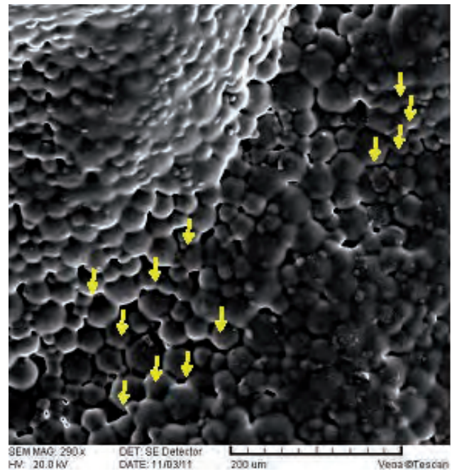
Figure 3b. Hexagonal crystallization of fluorapatite, FAP with characteristic 120 degree angles between the faces.
