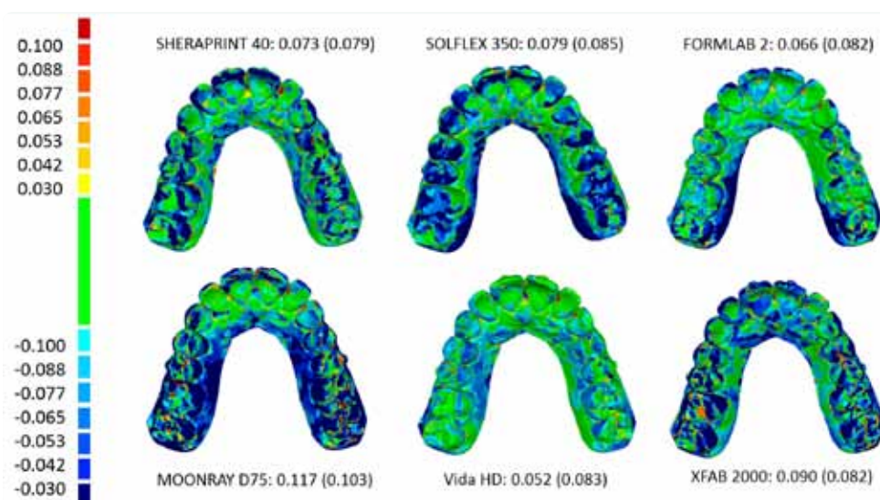
Figure 6: Mean trueness ( \pm SD), in mm, of the different 3D models 1 month after printing: best results obtained with each printer.
